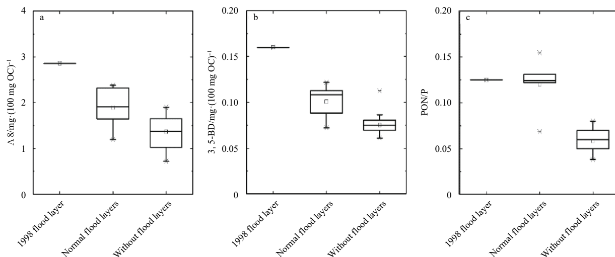
Fig. 7. \Delta 8 (a), 3, 5-BD (b) and PON/P (c) in different types of deposits in the TEZ core.
